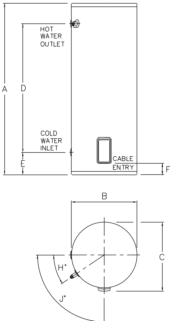
Dimensional Drawing Vulcan Domestic Electric
