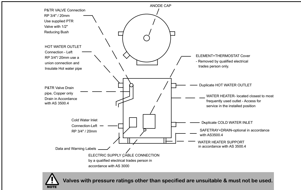
Figure 1 - Typical Installation of Water Heater
